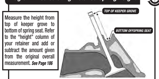
Diagram 1. Calculating Installed Spring Height
